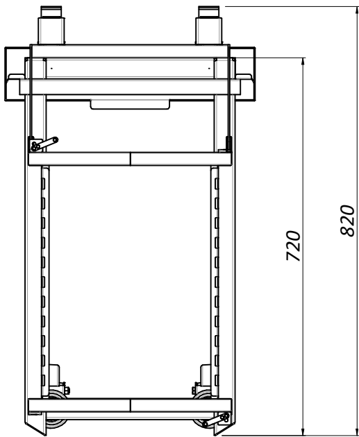
Capacity trolley
