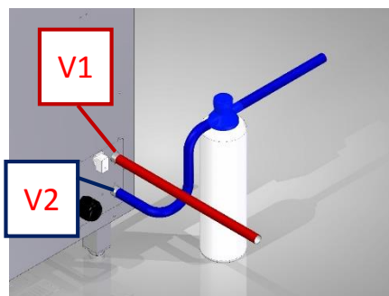
V1: Washing solenoid valve V2: Steam solenoid valve
